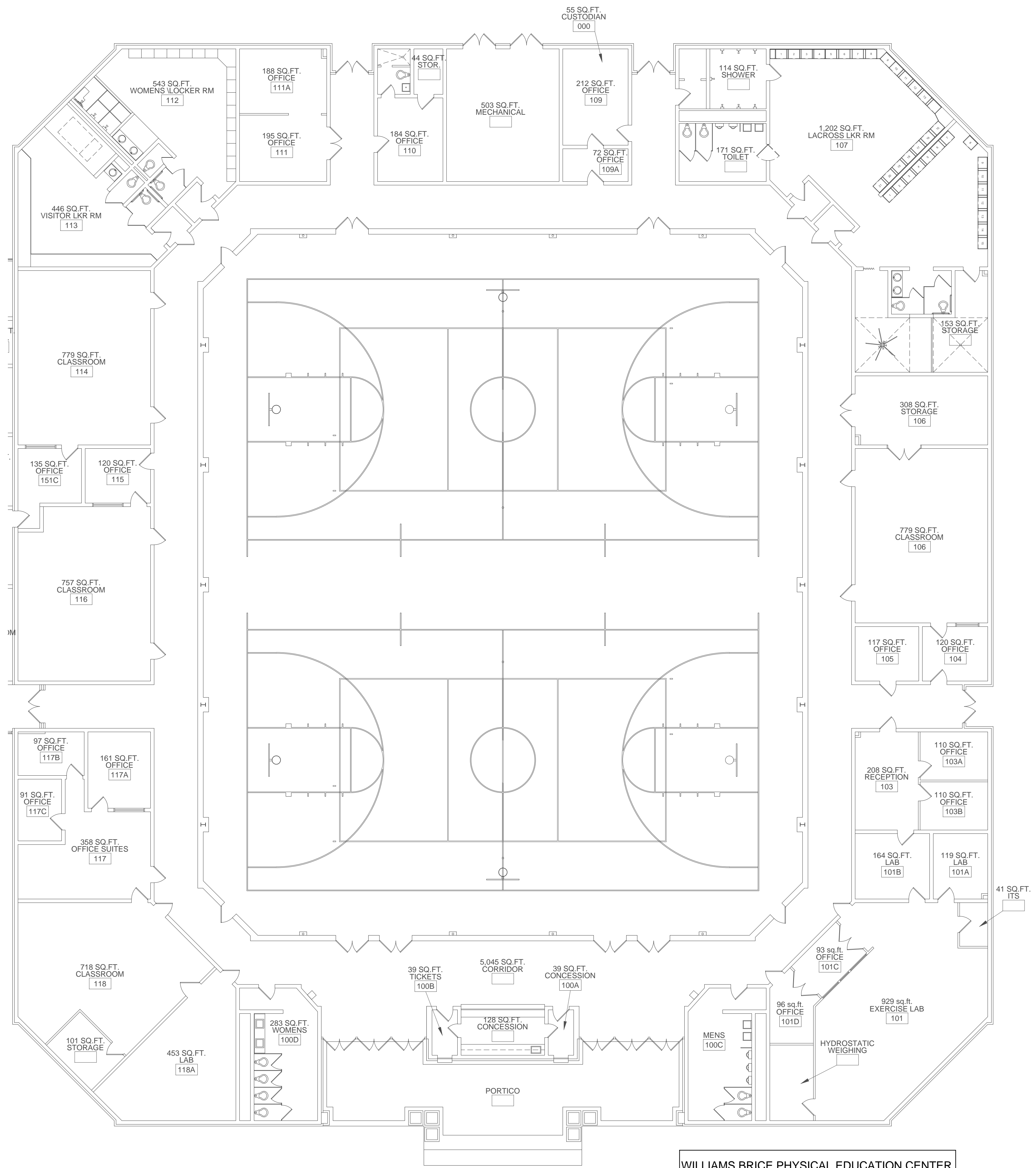
FLOOR PLAN SCALE: 1/16" = 1'-0"
